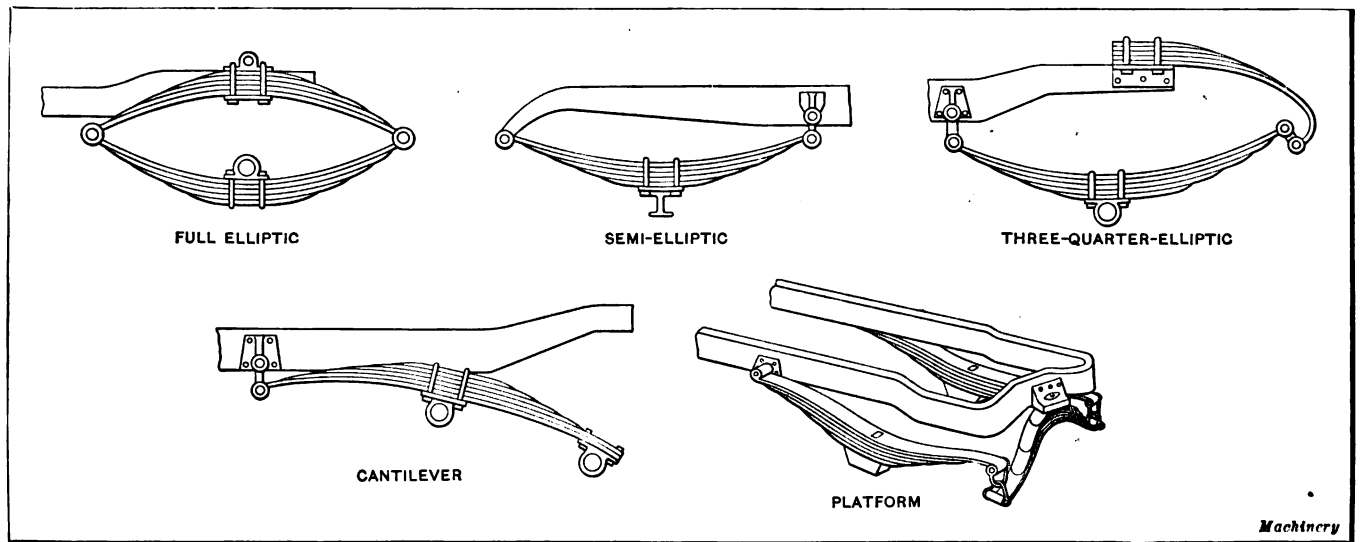
Fig. 1—Principal types of automobile springs
